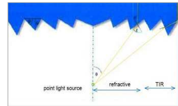
refractive structure and TIR-structure
